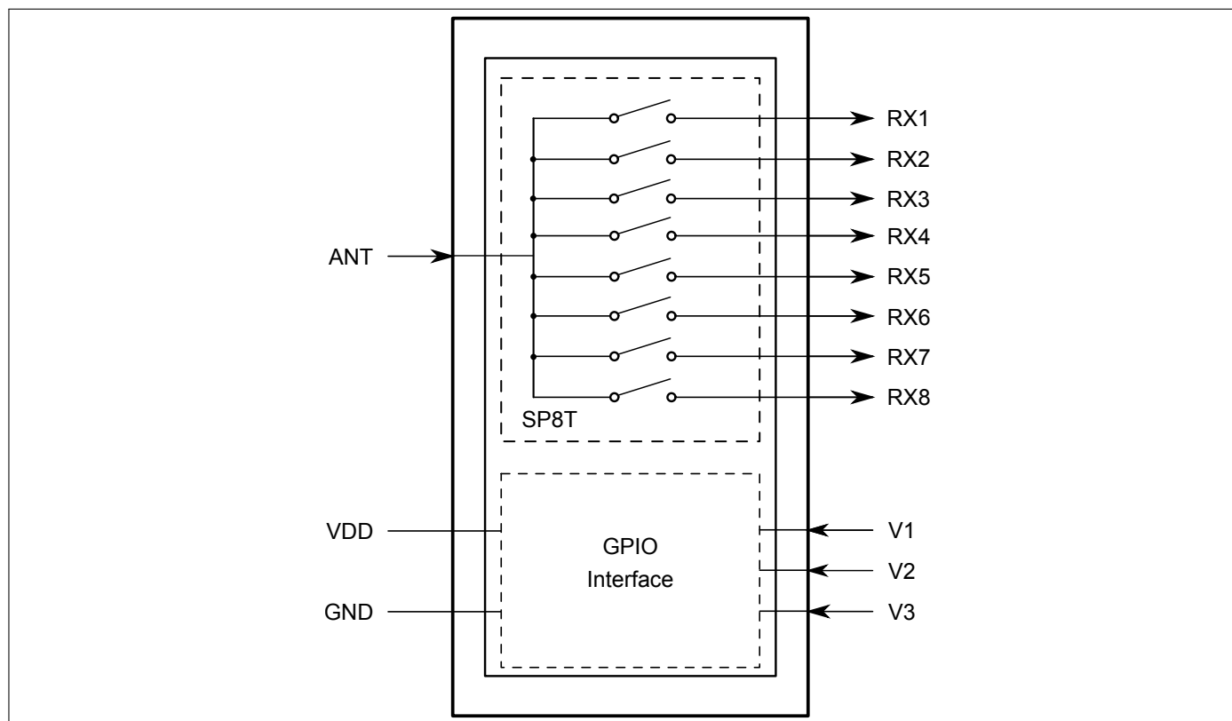
Figure 1: BGS18GA14 block diagram
